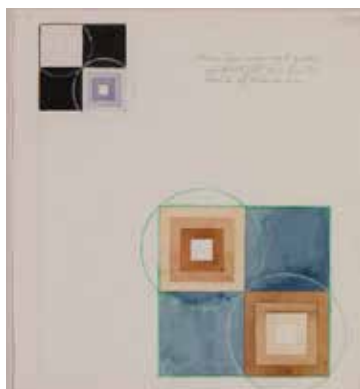
Fantasifulle atomer, 1917.
